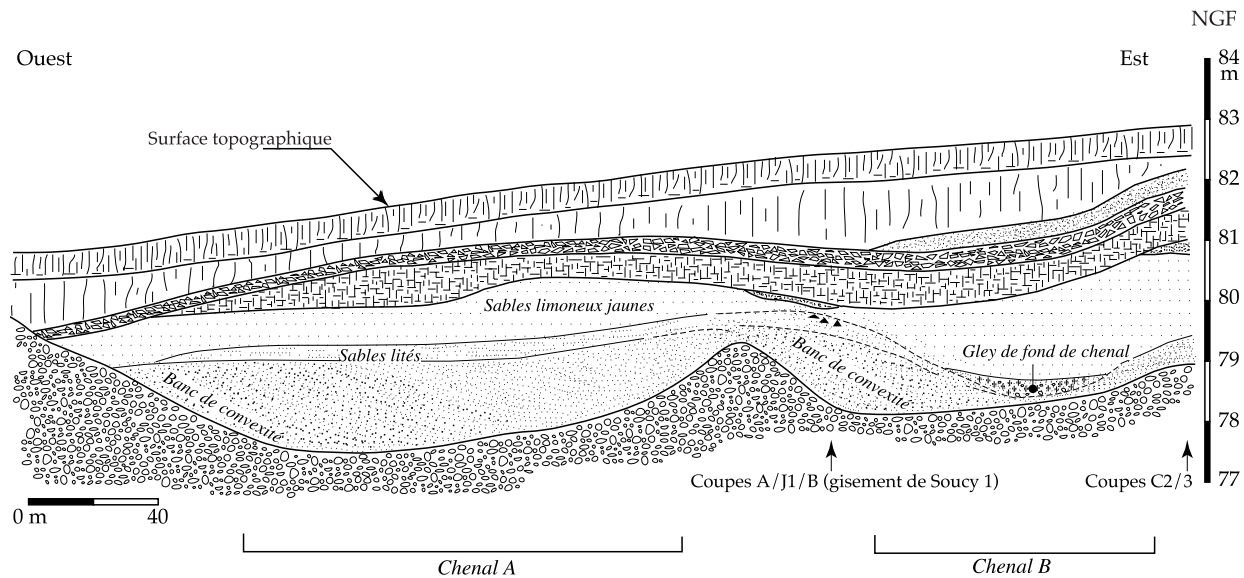
FIGURE 5. Transect est-ouest J de la plaine alluviale de Soucy-les-Grandes-Pièces. Localisation des coupes A/J1/B et C2/3. East-West transect J through the alluvial plain at Soucy-les-Grandes-Pièces. Location of sections A/J1/B and C2/3.
