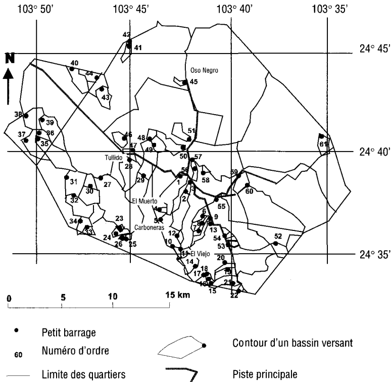
Figure 1 L'équipement hydrologique du ranch Atotonilco. The hydrological equipment in the Atotonilco ranch.
