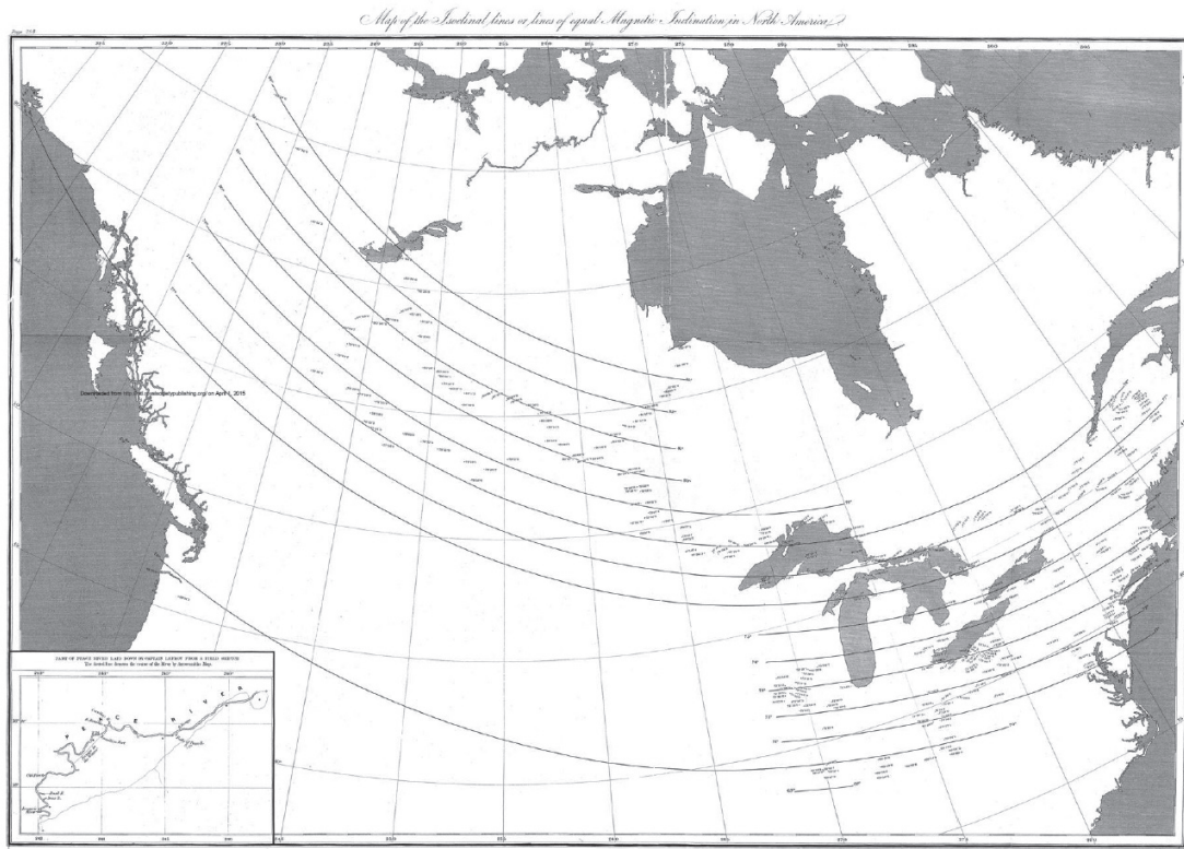
Figure 3. Map of the Isoclinal lines or lines of equal Magnetic Inclination in North America , in Edward Sabine, "Contributions to Terrestrial Magnetism, No. VII," Philosophical Transactions of the Royal Society 136 (1846): 258.
