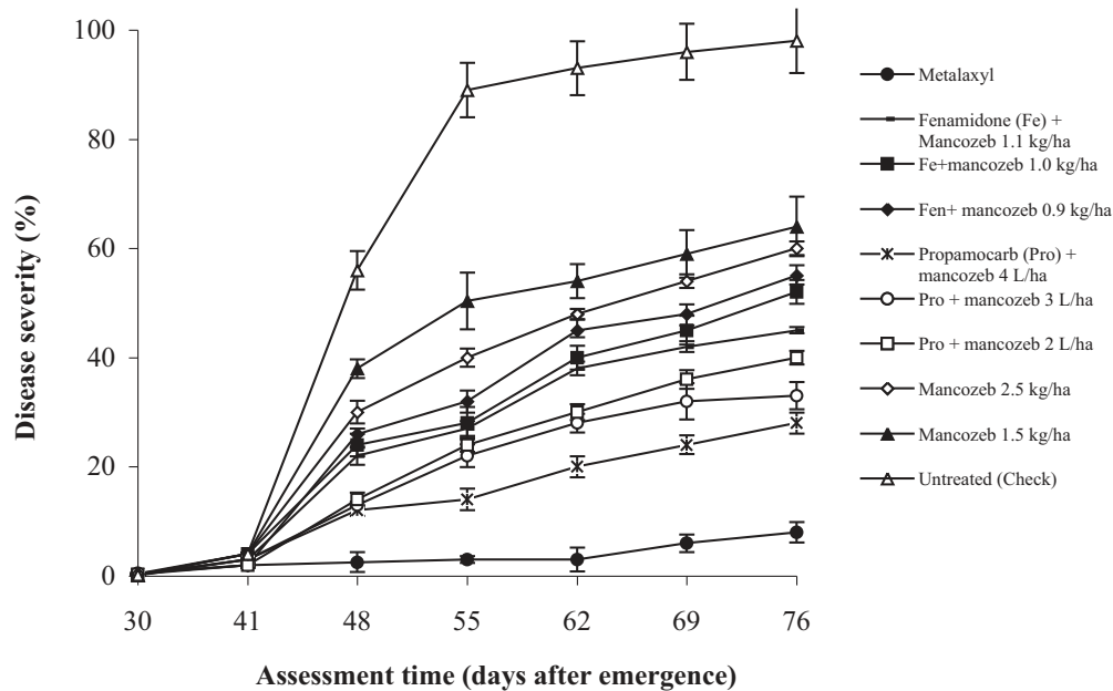
Figure 1. Progress of potato late blight ( Phytophthora infestans ) on cultivar Kerr's Pink treated with different fungicides at the Tigoni Research Station during the 1999-2000 cropping season. On each day of assessment, values = mean disease severity. The vertical bars represent standard errors of the mean.
