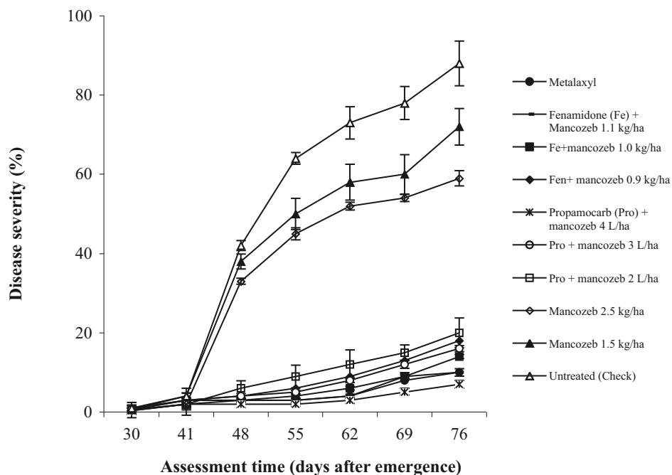
Figure 2. Progress of potato late blight ( Phytophthora infestans ) on cultivar Kerr's Pink treated with different fungicides at the Tigon Research Station during the 2000-2001 cropping season. On each day of assessment, values = mean disease severity. The vertical bars represent standard errors of the mean.
